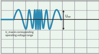
LV123/VW80303 Test pulse present voltage ripple
